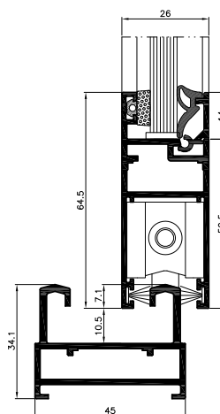
horizontally sliding window, view
